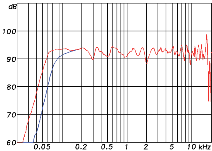
F 10 A Frequency response ( Low cut 50 / 110 Hz)
